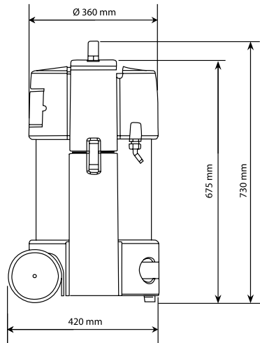
Dimensions Miniflex
